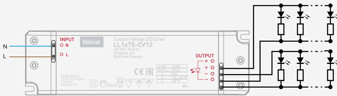
Parallel output connection
