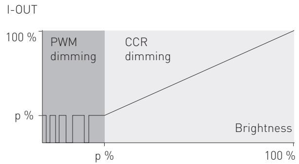
Hybrid dimming technique
