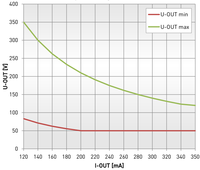
Output voltage U-OUT
